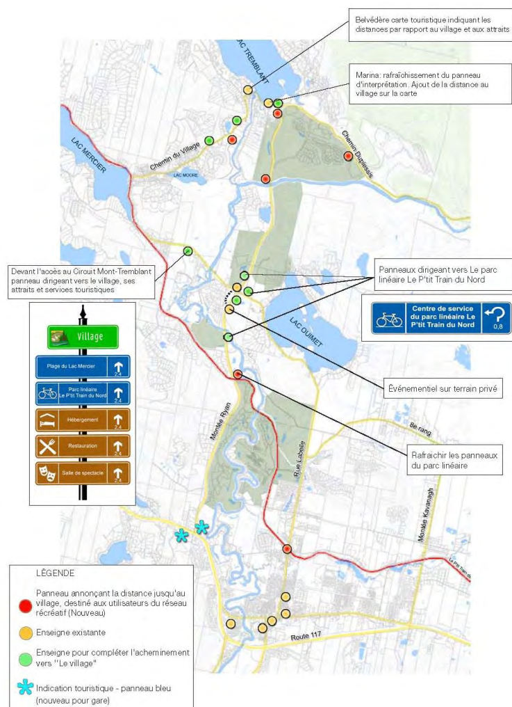
Figure 25 – Plan de signalisation
